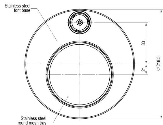
TOP VIEW SCALE 1:2
